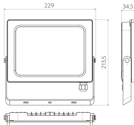
LD-VIPERS50W-40
