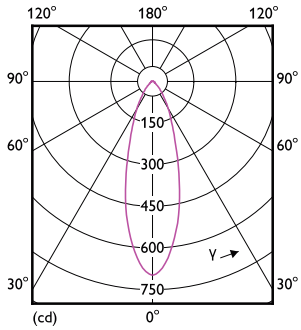
LEDspots Corepro SLR 4W PAR16 GU10 840 36D-LDD
