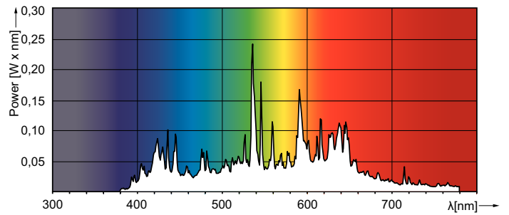
LDPO_CDMTC-E_0007-Spectral power distribution Colour
