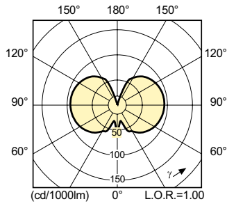
LDLD_CDMTC-E_0007-Light distribution diagram
