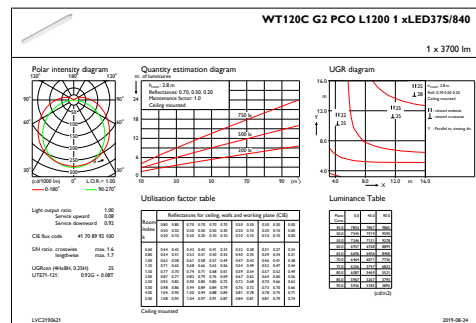
IFGU1_WT120CG2PCOL12001xLED37S840
